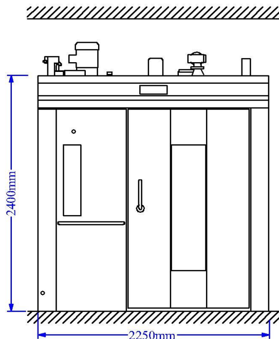
VISTA FRONTAL
