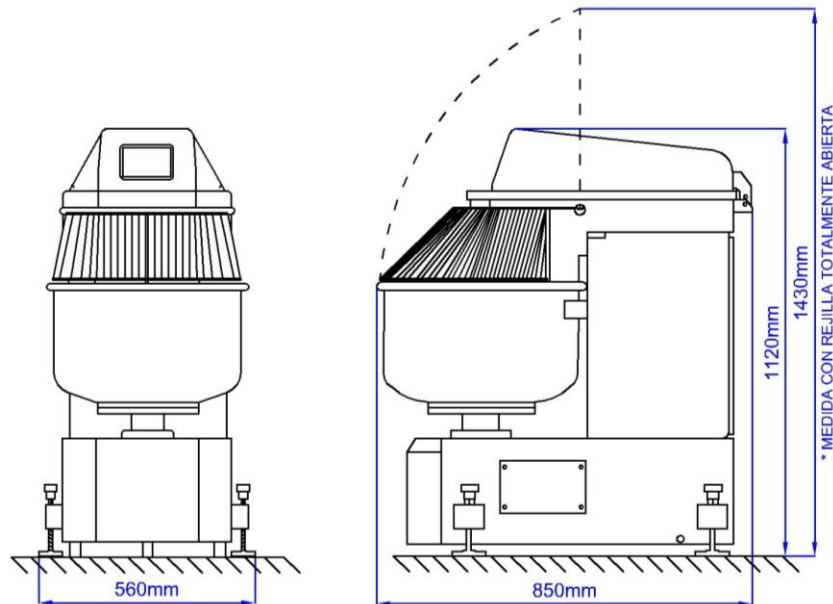
VISTA FRONTAL
