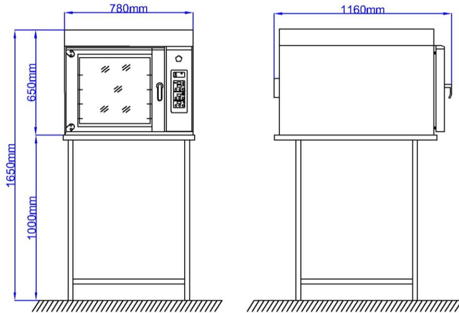
VISTA FRONTAL
