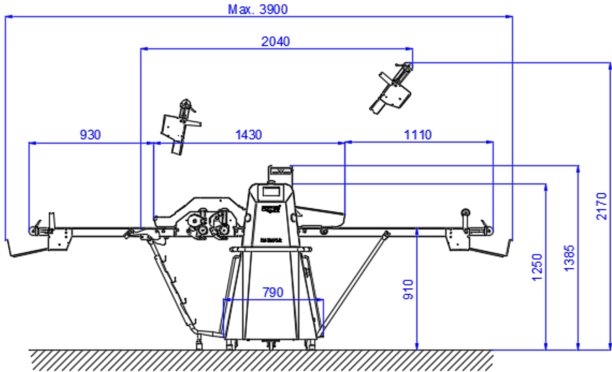
VISTA FRONTAL
